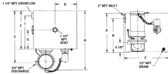
G series (simplex) 8 or 15 gallon tank
