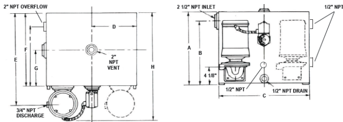
G series 30-120 gallon tanks
