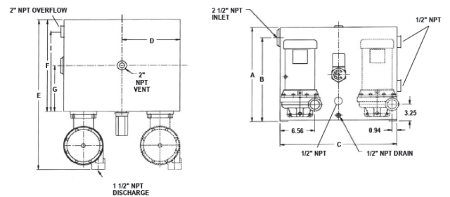
J series 30-120 gallon tanks
