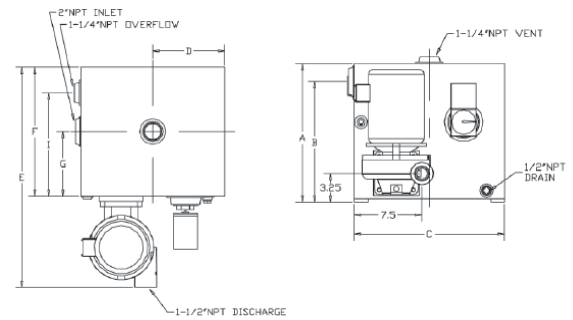
J series 30-120 gallon tanks
