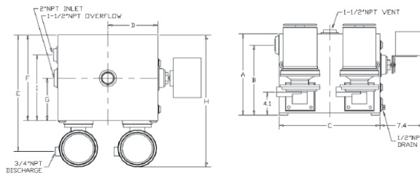
G series (duplex) 15 gallon tank
