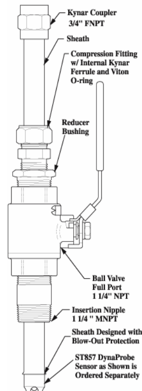
Model SA857 Valve Retraction Sensor Housing
